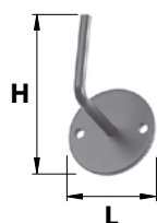
OMC80.. Support de main courante 80
